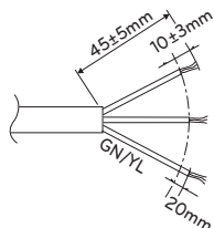
<Sheath-removal guide>
