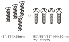
4 x Stand screws
