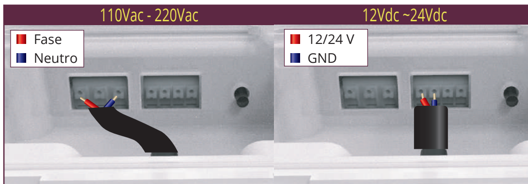
Figure 1 - Connection terminals
