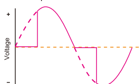
Forward-phase control dimmer
