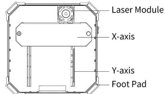
04 Bottom View
