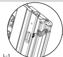
L-1 (GS0201016) Crosshead screw Q2540410 M4x10x2pcs
