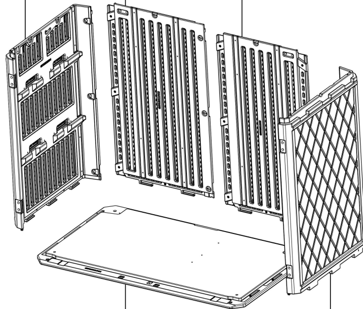
Right side panel (GS0201005)
