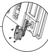
Latch-1 (GS0201018)x1pcs
