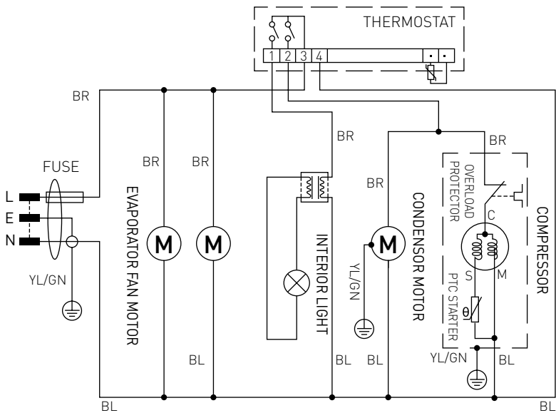
Circuit diagram (235829)
