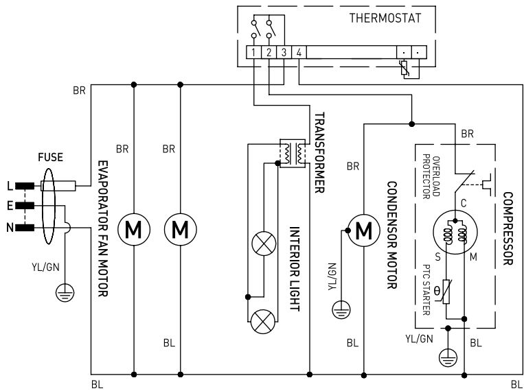
Circuit diagram (233931)
