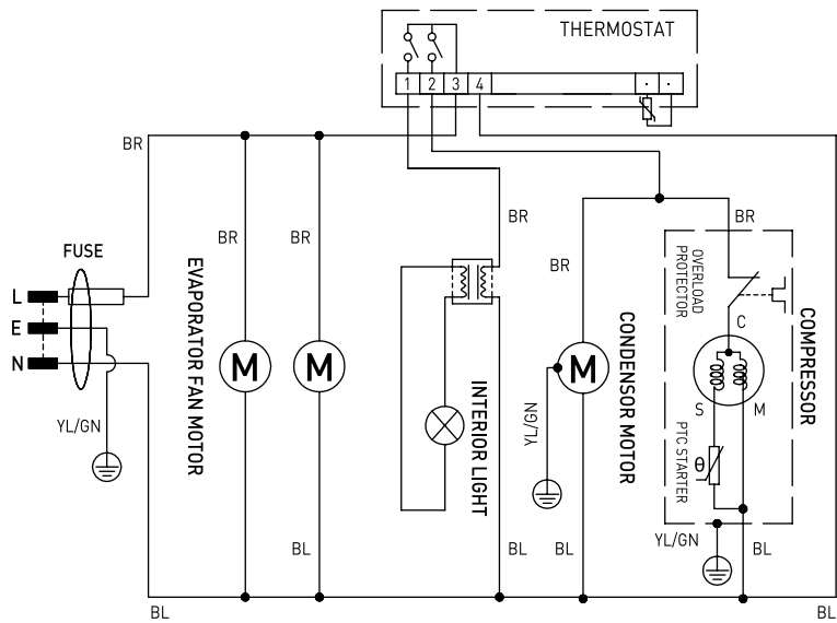
Circuit diagram (233924)
