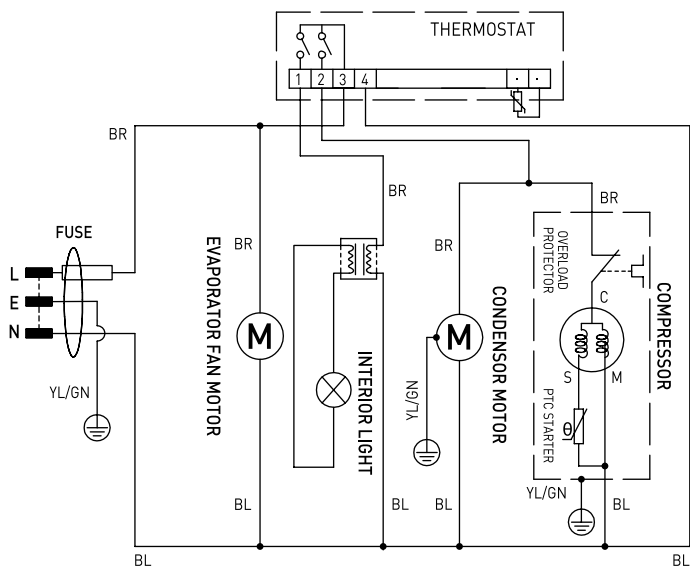
Circuit diagram (233900)
