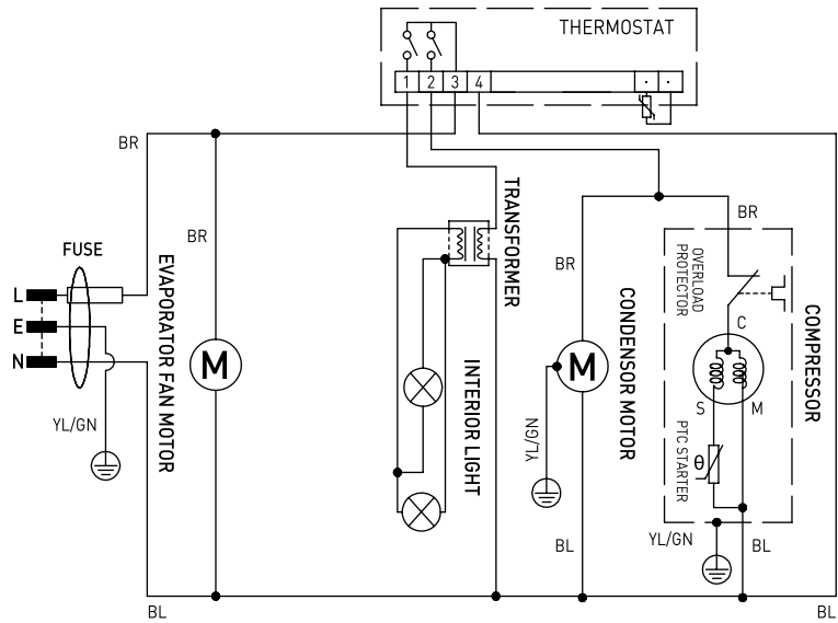
Circuit diagram (233924)
