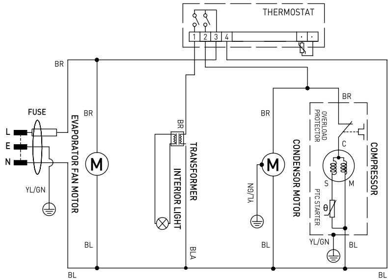
Circuit diagram (233900)
