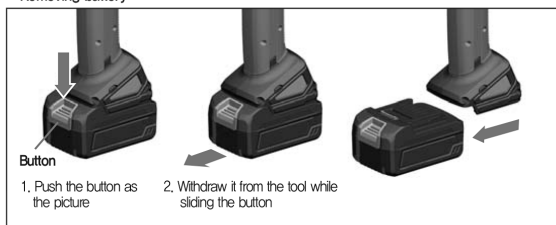
– Removing battery
