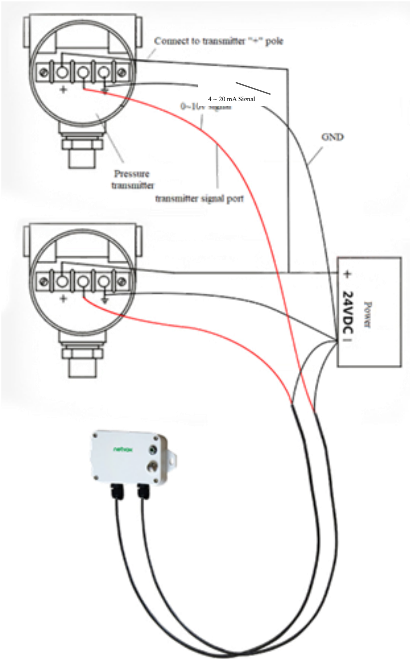
3-wire System Example Diagram (for wiring reference)
