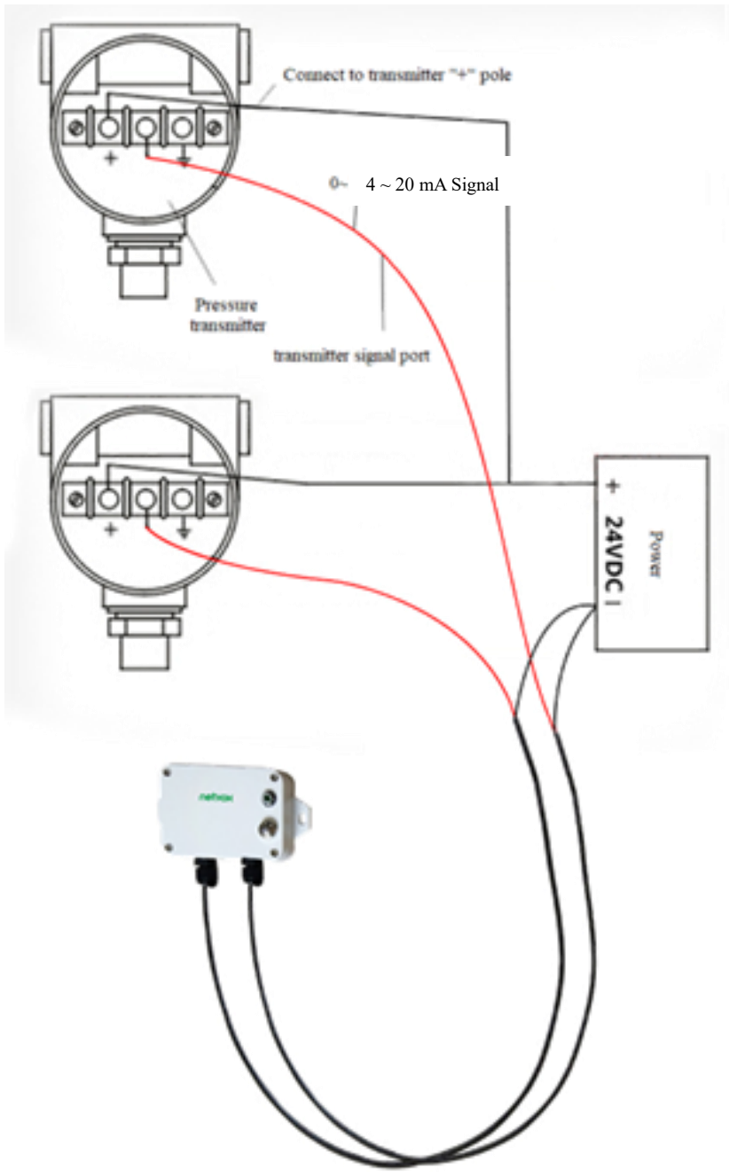
2-wire System Example Diagram (for wiring reference)
