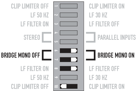
Channel 2 settings, switches 8, and 10 are set to off.
