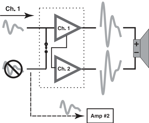
Channel 2 Can Be Used to Daisy-chain to Other Amplifiers. – Figure 22 –
