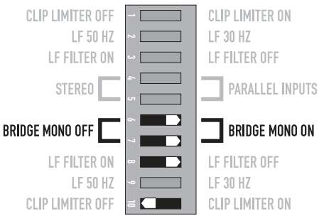
Set Channel 2 dip switches, 8 and 10, to off. – Figure 20 –
