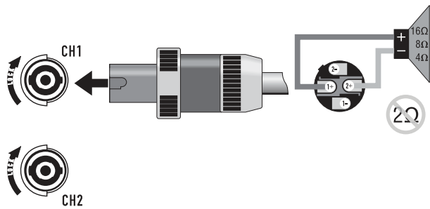
Bridge Mono Mode – Figure 31 –
