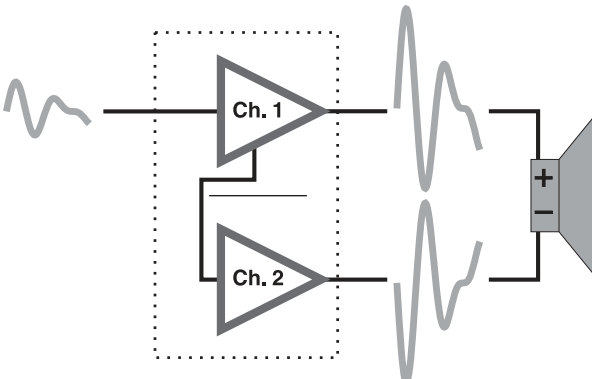
Channel 1 Input, Channel 2 Not Used – Figure 21 –
