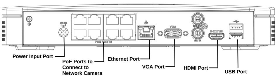
Figure 3 RVNVR080020 NVR Components
