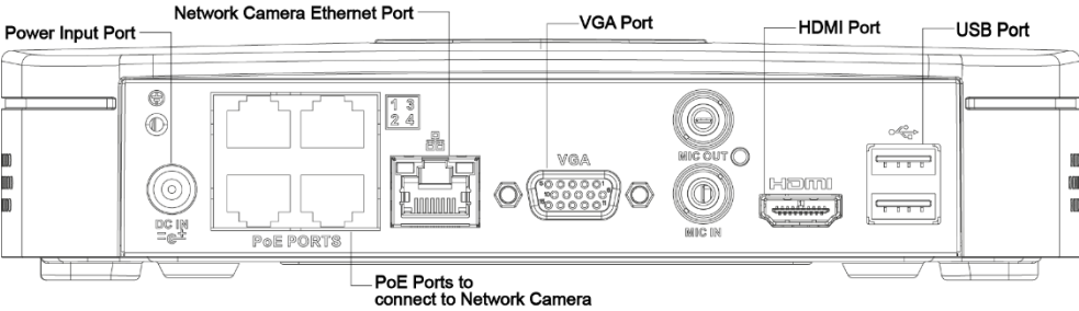
Figure 2 RVNVR04002P Components
