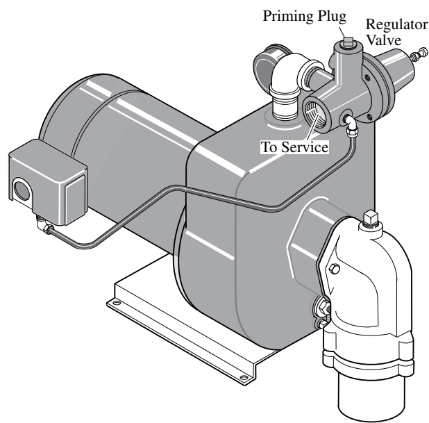
Figure 2 – Well Casing Adapter bolted directly to pump
