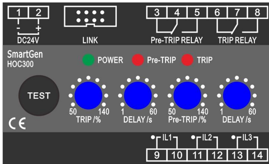
Fig.1 – Panel Drawing
