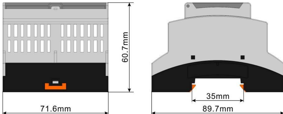
Fig.7 – Case Dimensions and Cutout
