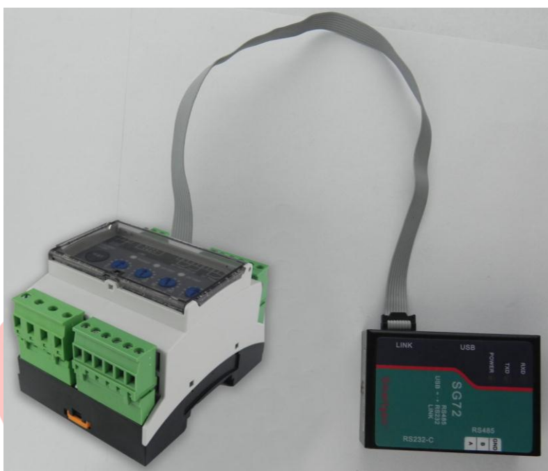
Fig.2 – PC Program Connection
