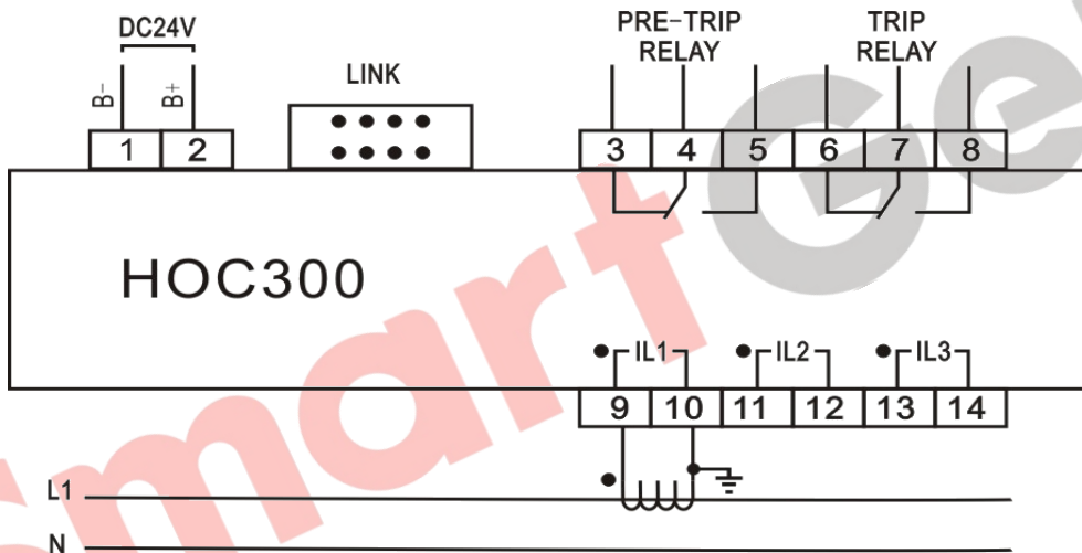
Fig.6 - Single Phase 2 Wire Typical Application
