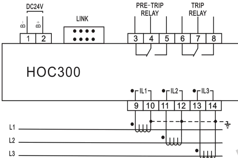
Fig.3 - 3 Phase 4 Wire Typical Application
