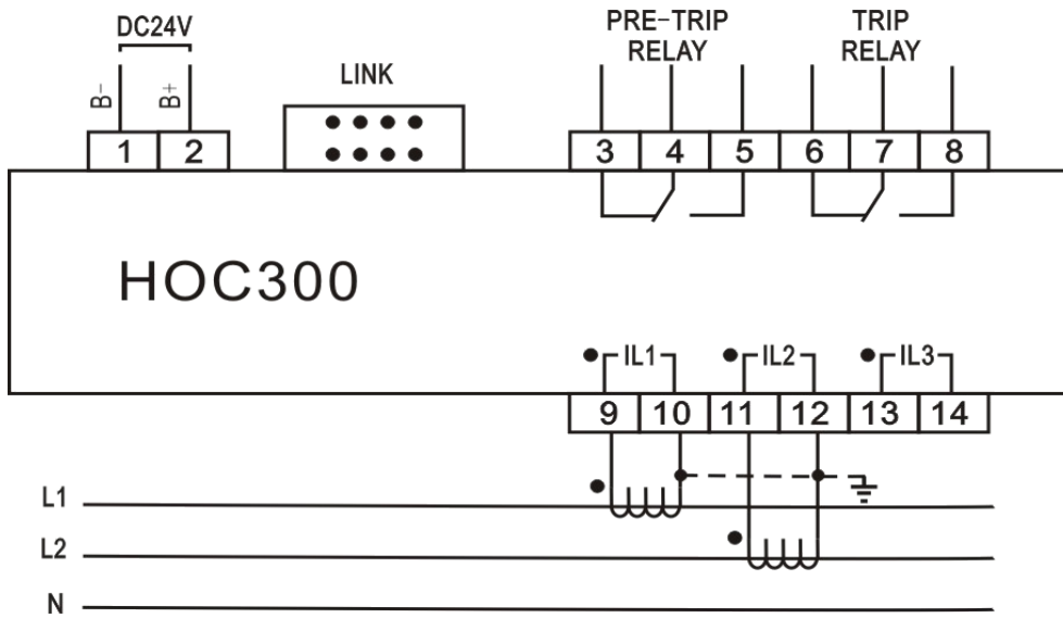
Fig.5 - 2 Phase 3 Wire Typical Application
