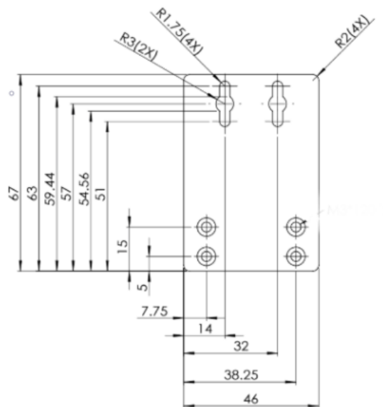
Figure 3.5: Wall Mounting Bracket Dimensions
