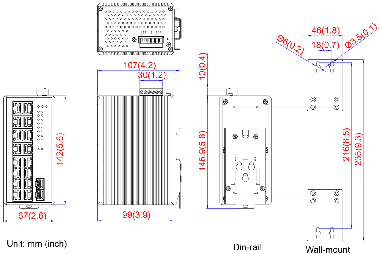
Figure 2.1: Physical Dimensions
