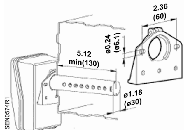
Figure 3. Mounting Flange.
