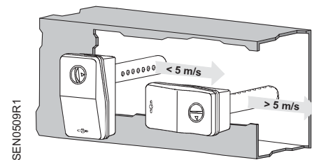
Figure 2. Mounting Orientations.
