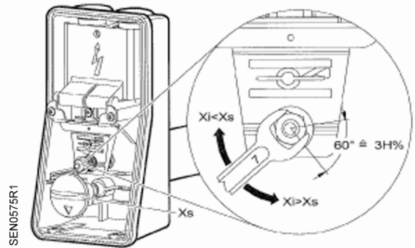
Figure 5. Humidity Calibration.
