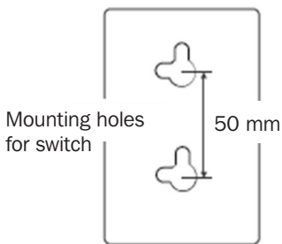
Mounting Holes Drawing of NGI-U05
