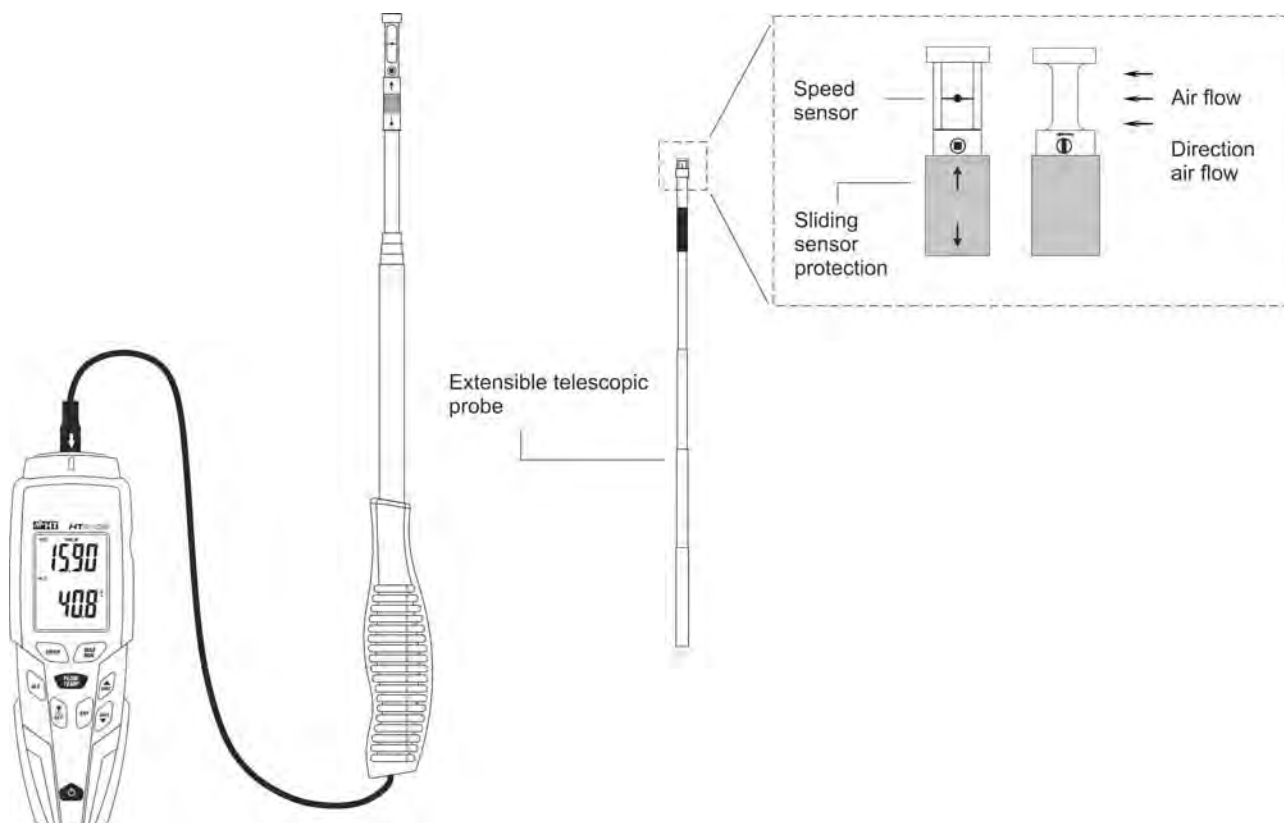
Fig. 7: Measurement of air speed and temperature
