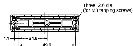
G7SA-3A3B Mounted
