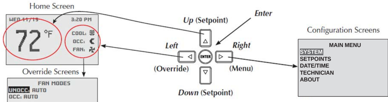
FIGURE 2 CompleteStat Buttons and Home, Override and Configuration Screens
