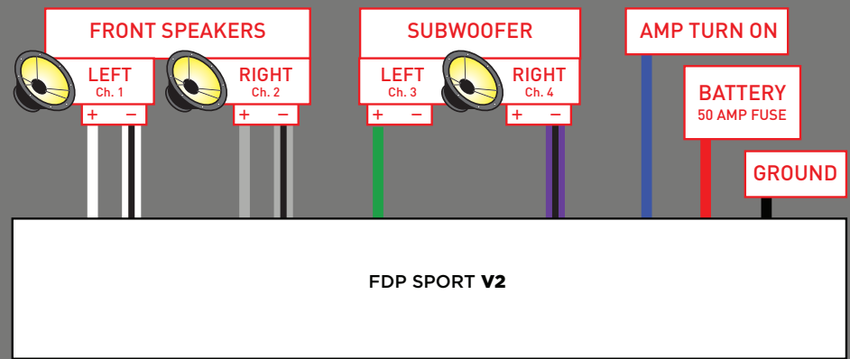
Figure 4B | 3 Channel Stereo & Bridged Mode Wiring Diagram
