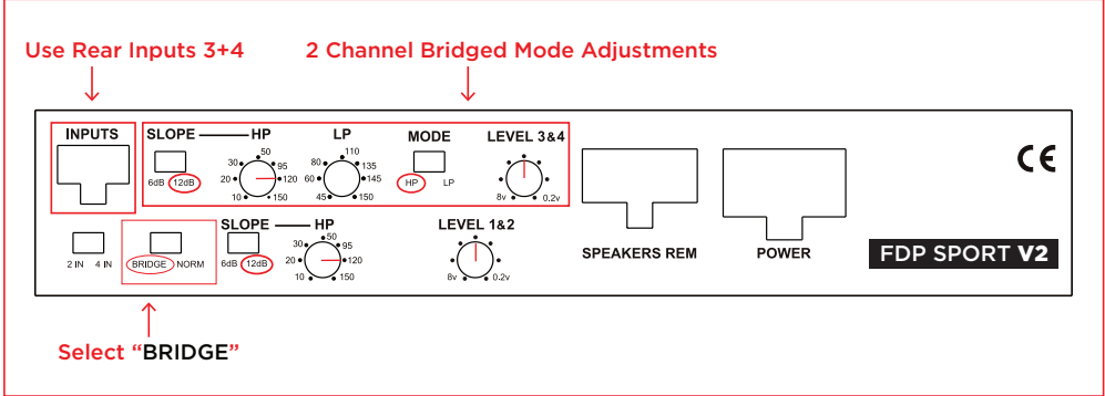
Figure 3B | 2 Channel Bridged Stereo Mode Wiring Diagram
