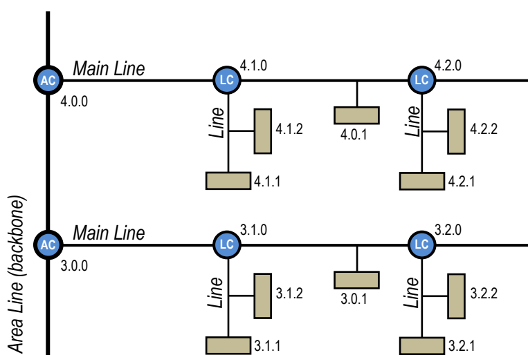
Figure 3 Line Coupling
