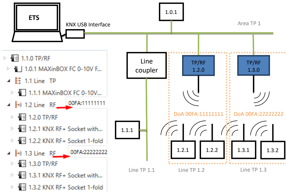
Figure 4 Example of a TP + RF mixed installation
