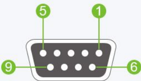
RS232 PINOUT
