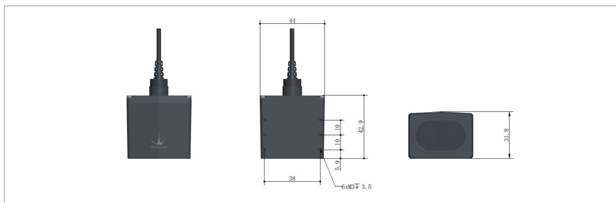
TF03-100 dimensions (Left 1: top view; Left 2: upward view; Left 3: front view)
