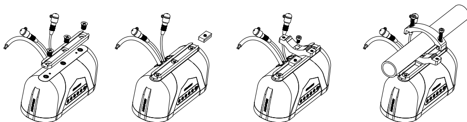
Attach bracket to desired mounting location using provided screws
