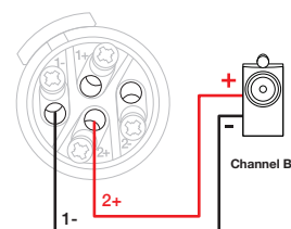
Bridge-Tied Load Wiring
