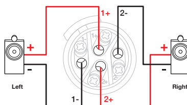
Single Wiring
