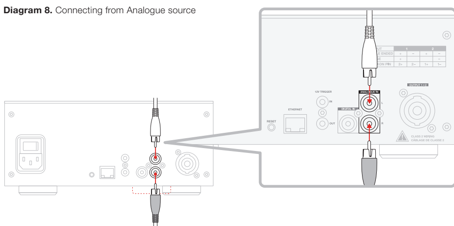
Diagram 8. Connecting from Analogue source
