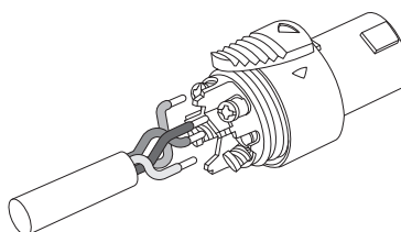
Bridge-Tied Load Wiring
