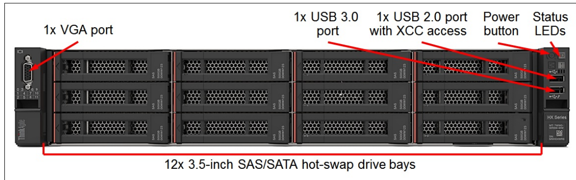
Figure 2. HX5521-C front view
