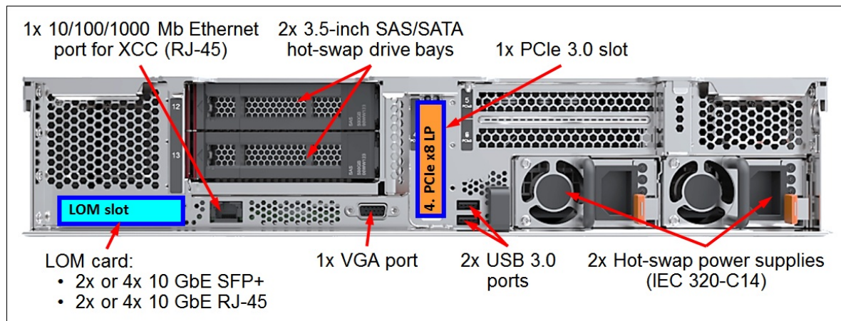
Figure 4. HX5521-C 14-drive bay node rear view
