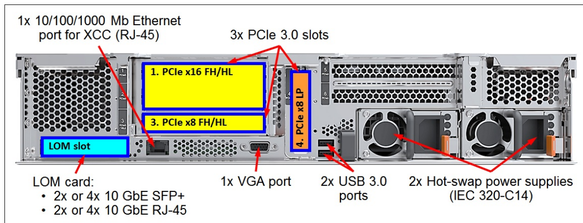
Figure 3. HX5521-C 12-drive bay node rear view
