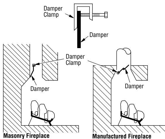
Figure A - Attaching Damper Clamp
