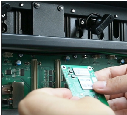
Figure 37: Remove Receiver Card from Hub Board
