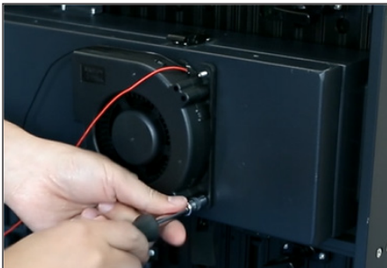
Figure 45: Remove Screws Securing Fan to Power Box
