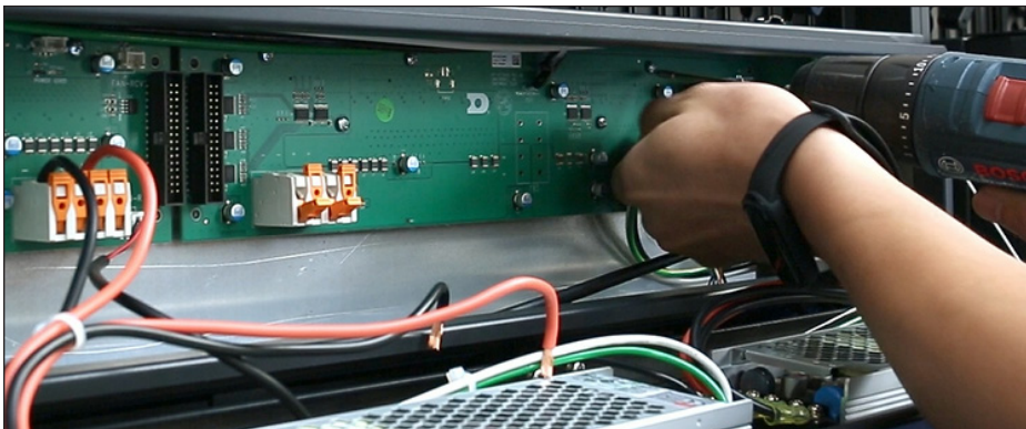
Figure 42: Remove Screws Securing Hub Board to Power Box
