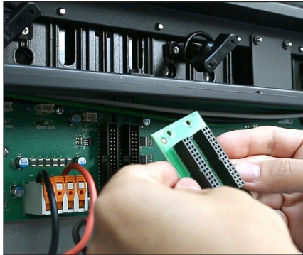
Figure 40: Remove Jumper Board Connecting Hub Boards Together
