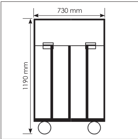
Figure 6: Flight Case (Side View)
