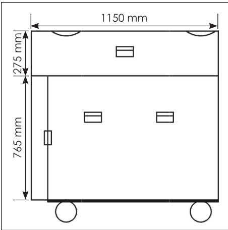
Figure 5: Flight Case (Front View)
