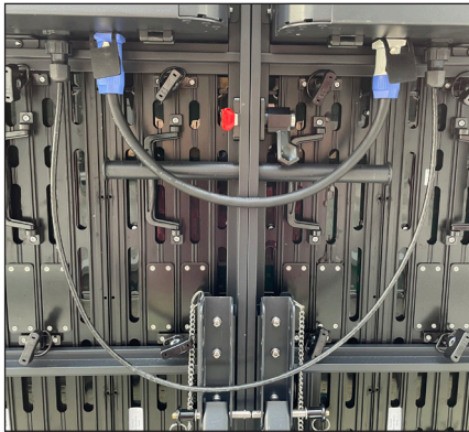
Figure 17: Route Cables Left to Right
