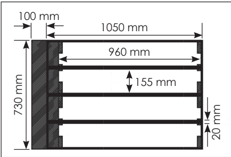
Figure 7: Flight Case (Top View)
