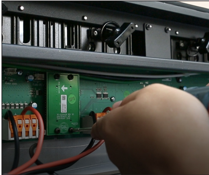
Figure 39: Remove Screws Securing Jumper Board to Hub Board
