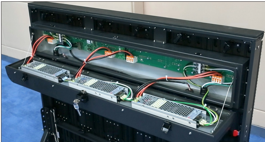
Figure 46: Power Supplies in Power Box
