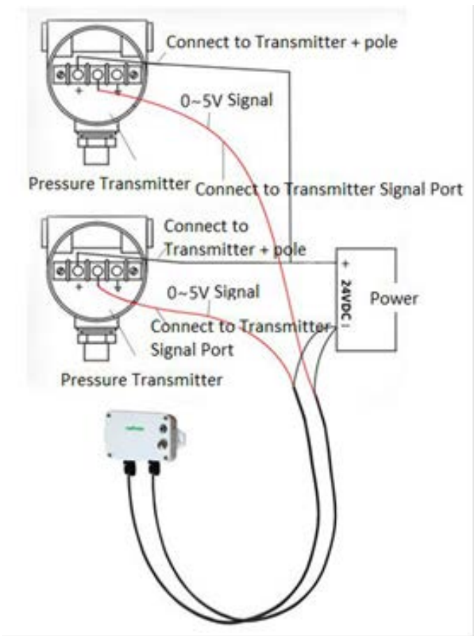
Fig. 2-wire System Example Diagram (for wiring reference)
