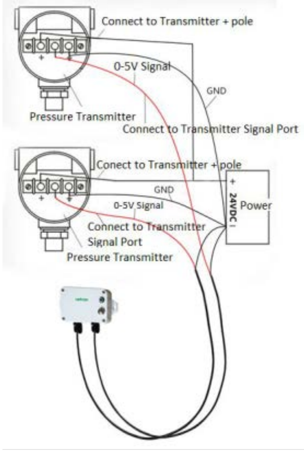
Fig. 3-wire System Example Diagram (for wiring reference)
