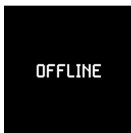
Figure 7: Offline screen
