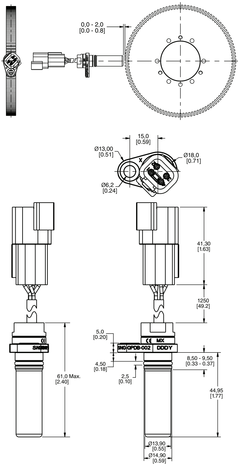
Figure 8. SNG-QPDB-002 Mounting Dimensions (For reference only: mm/[in].)
