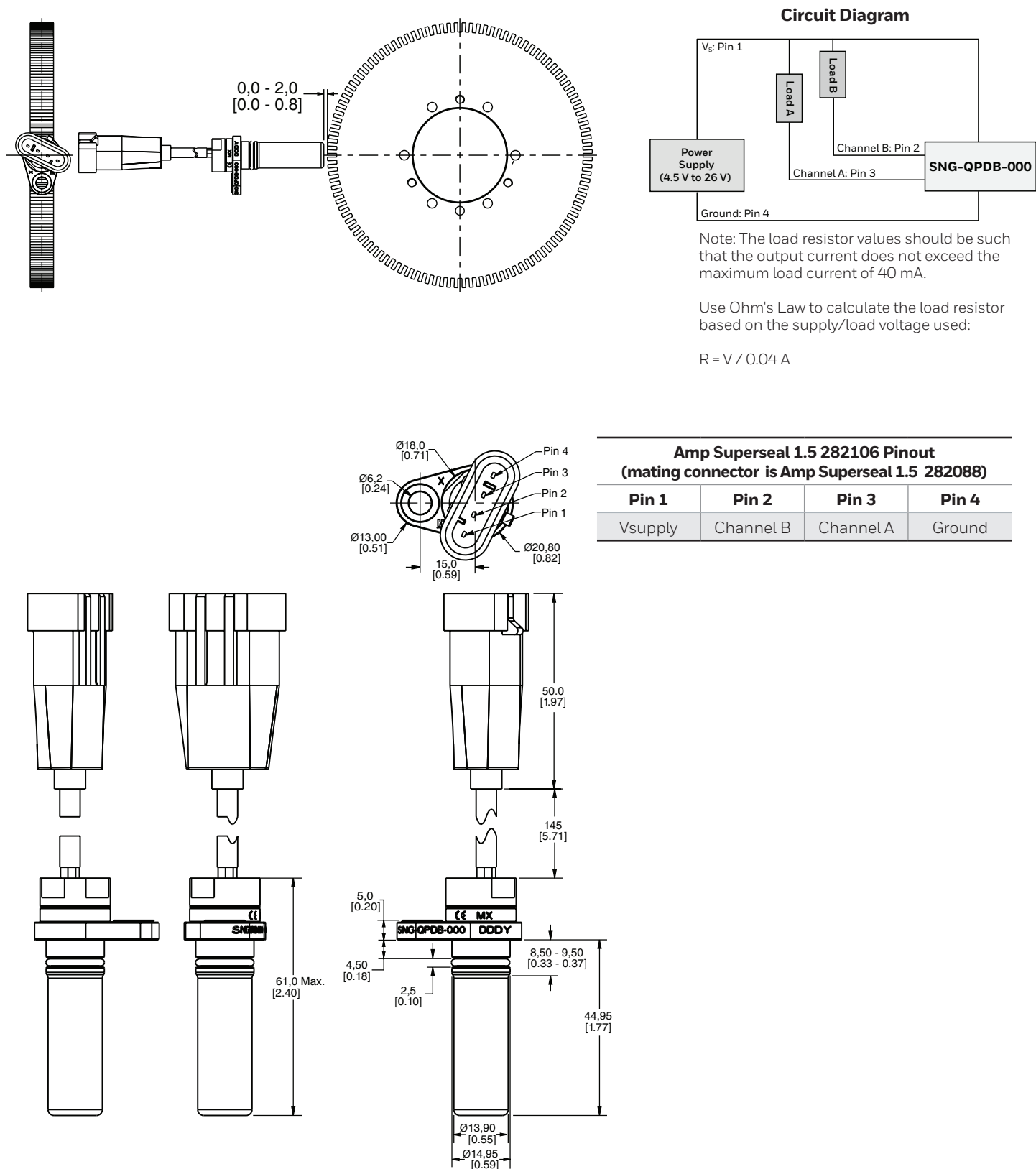
Figure 7. SNG-QPDB-000 Mounting Dimensions (For reference only: mm/[in].)
