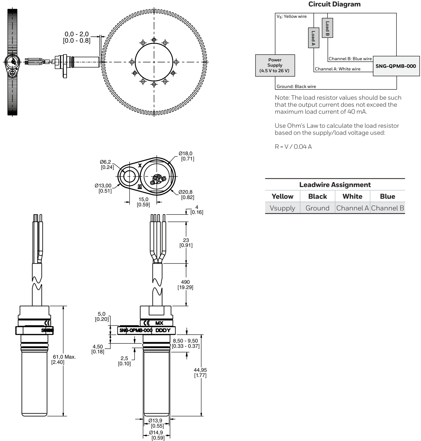
Figure 6. SNG-QPMB-000 Mounting Dimensions (For reference only: mm/[in].)
