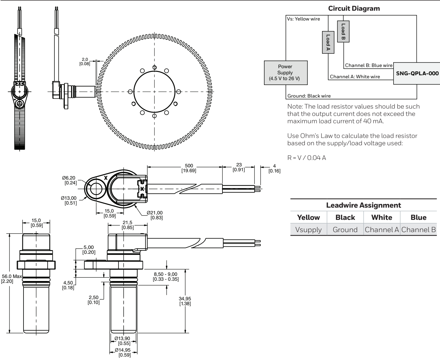
Figure 3. SNG-QPLA-000 Mounting Dimensions (For reference only: mm/[in.] )
