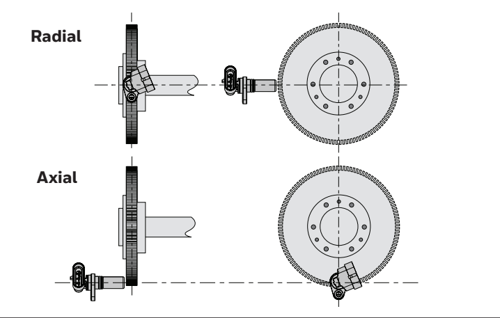
Figure 2. Possible Mounting Orientations
