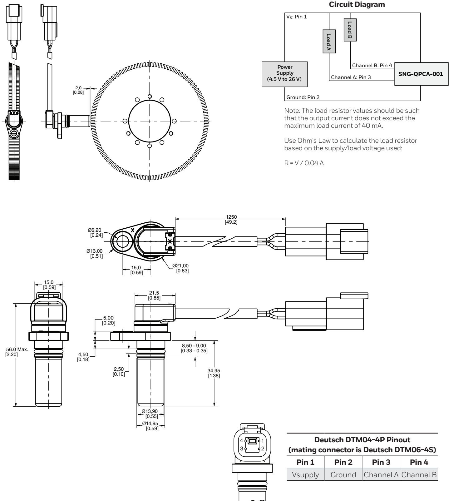
Figure 4. SNG-QPCA-001 Mounting Dimensions (For reference only: mm/[in].)
