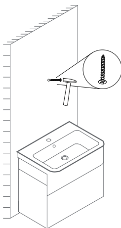
5.Drive a screw into the hole.
