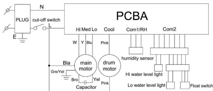
Wiring diagram
