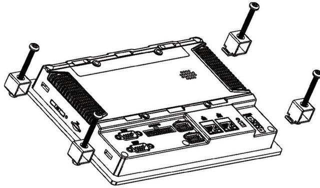
Embedded mount
