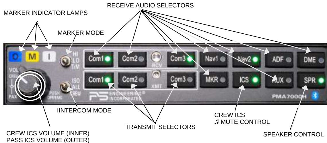
Figure 3-1 PMA7000H-BT controls
