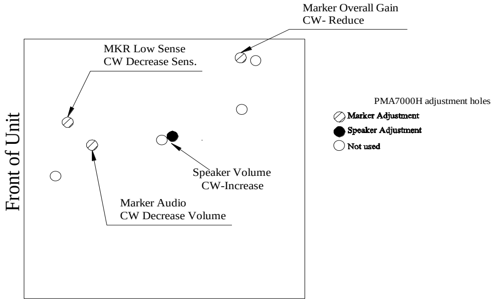
Figure 2-3- PMA7000H-BT Adjustments
