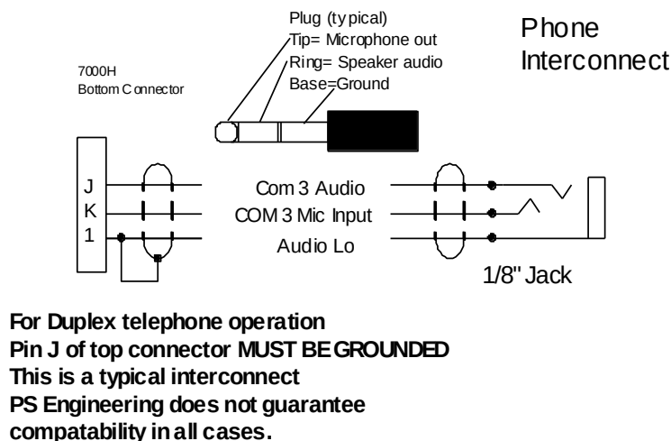
Figure 2 -2 Duplex Telephone interface
