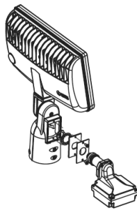
DSXF2 (Integral slipfitter with rSBOR)
