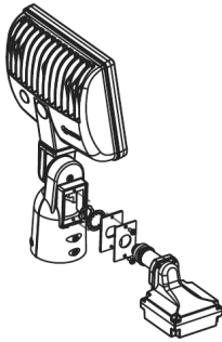
DSXF1 (Integral slipfitter with rSBOR)
