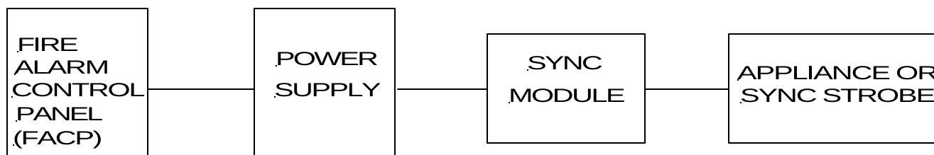
Figure 1: SM Connection Diagram with Power Supply
