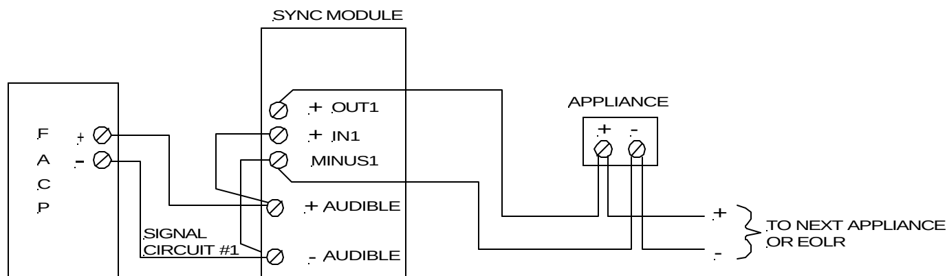
Figure 3: Class “B” Circuit without Audible Silence Feature. Red and Black Shunt Wires are Supplied.
