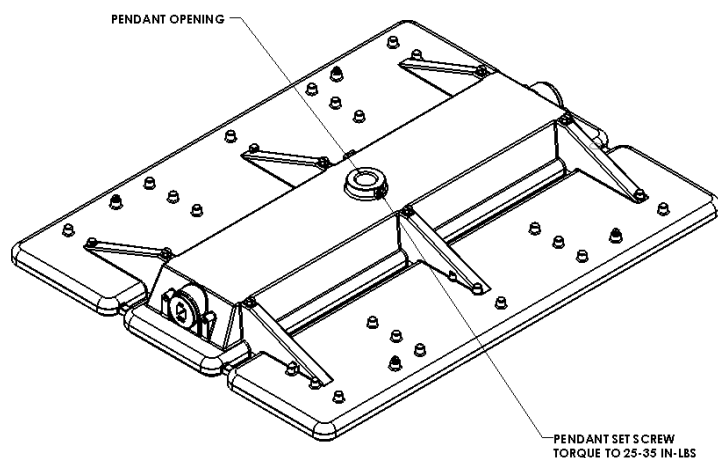
Figure F.1: 24L Pendant Mount Location
