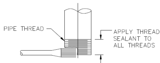
Figure F.4: Detail View of Application of Thread Sealant
