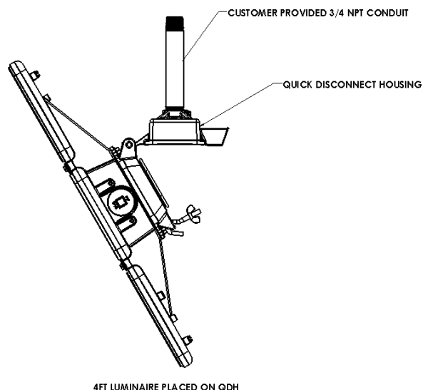
Figure F.2: 48L Pendant Mount
