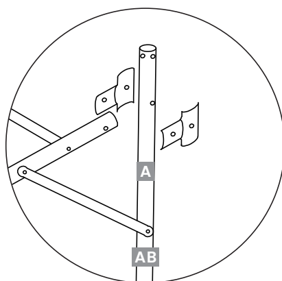
POSITION 1: H1880MM
