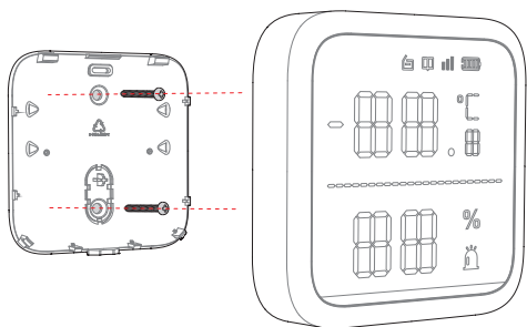
Screw Mounting
