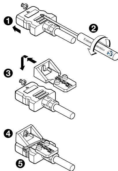
Figure 2. Securing the HDMI Connector
