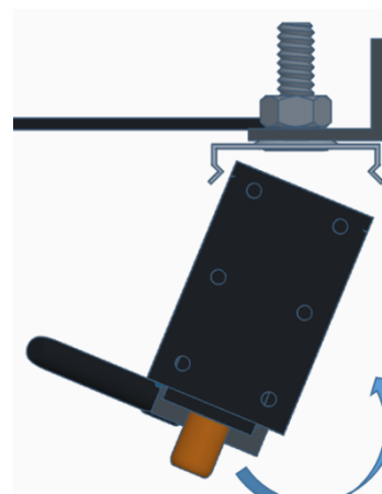
Vertical Rack Mount Step 3
