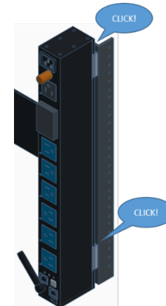
Vertical Rack Mount Step 2
