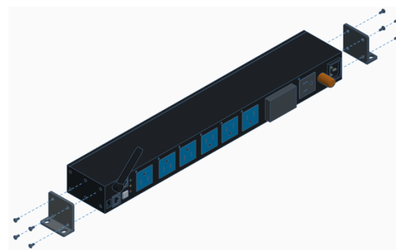
Surface Mount Step 1
