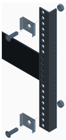
Vertical Rack Mount Step 1
