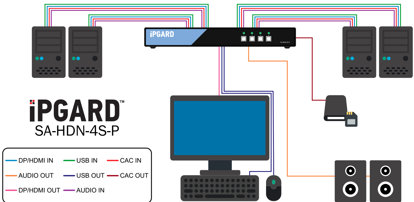
Figure 6-1: SA-HDN-4S-P
