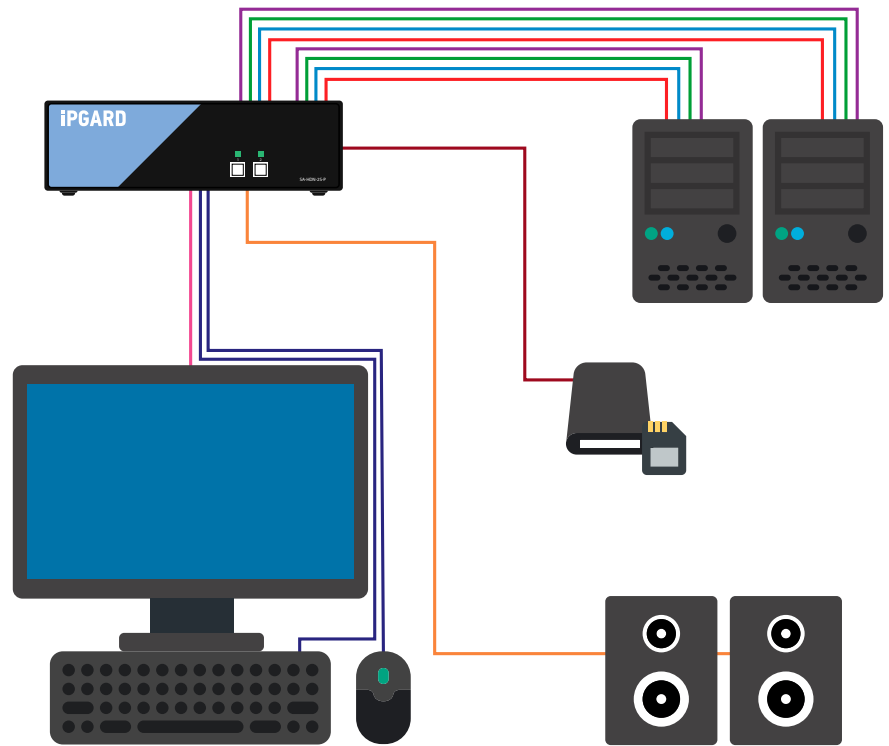
Figure 8-1: SA-HDN-2S -P
