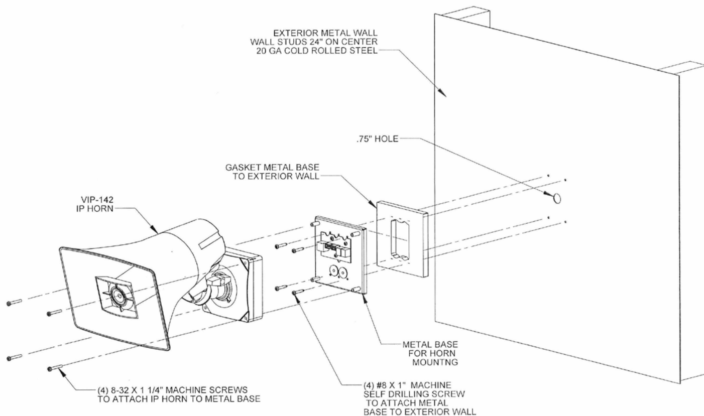
Figure 4. Exterior Mounting
