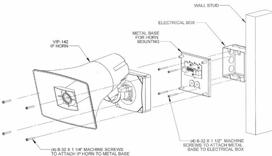
Figure 3. Interior Mounting
