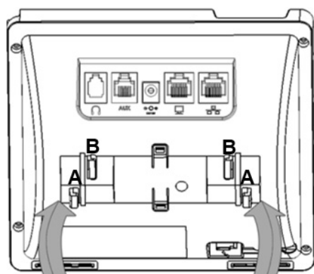
Desk Mount
