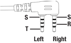
Figure 7: 3.5 mm Dual Mini (Gold) TRRS Connector
