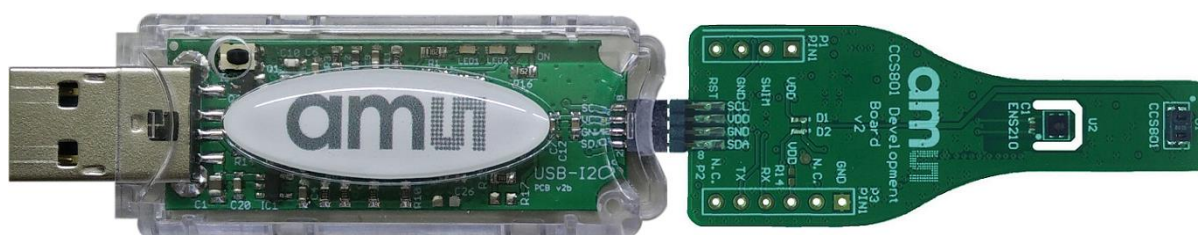
Figure 1 CCS801 sensor shield with USB-I2C dongle
