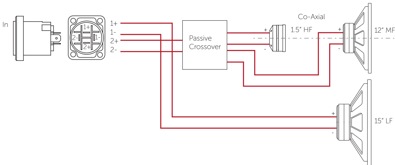
Figure 4.1: Wiring diagram
