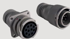
Cannon VG95234 (CA Bayonet) with Tin Zinc J Plating
