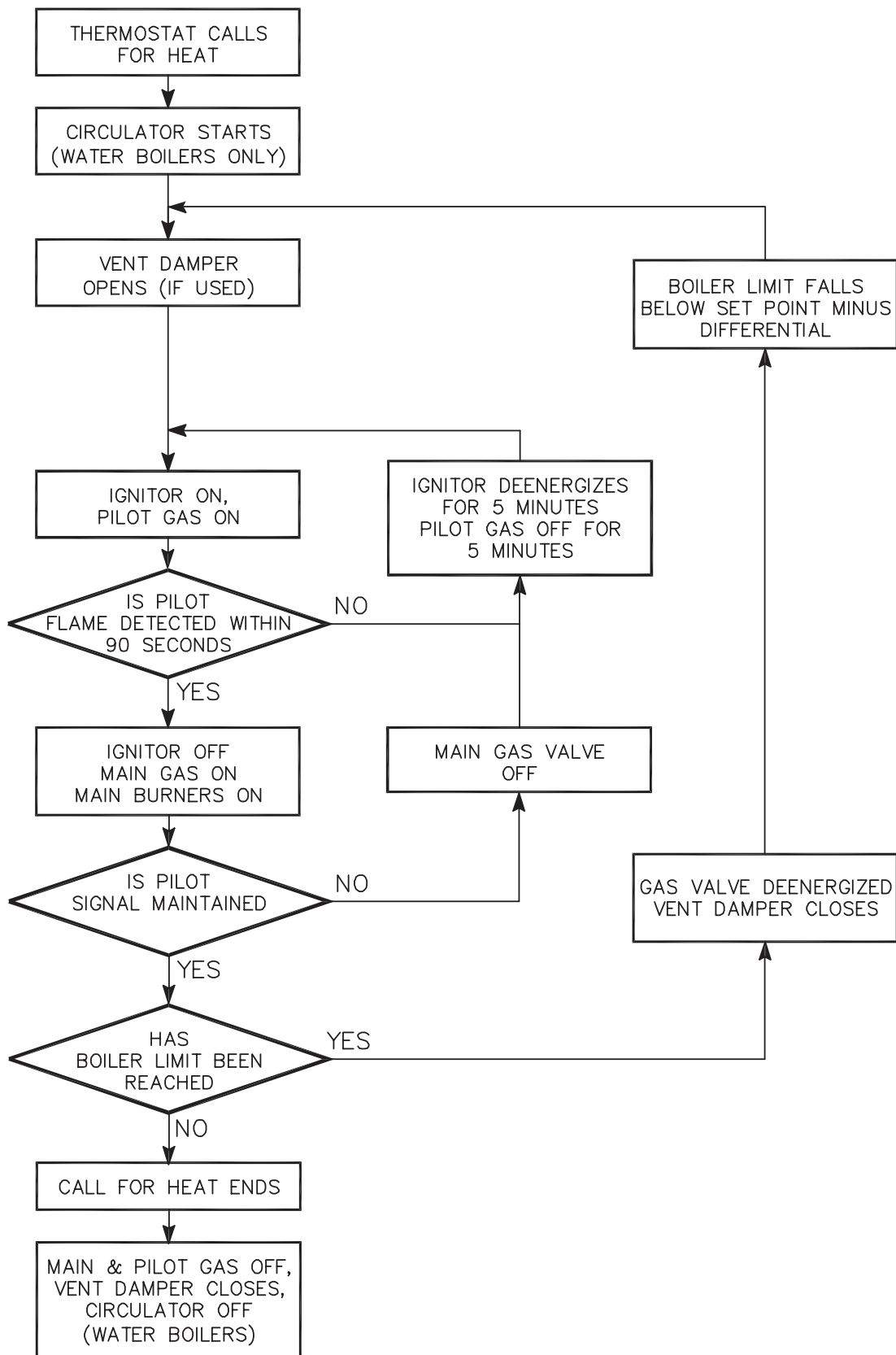
Figure 2: Sequence of Operation
